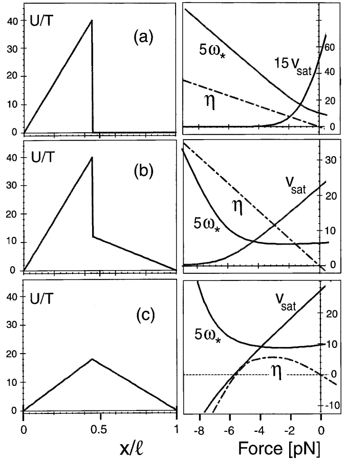
Fig. 2a–c Left column Molecular interaction potentials U \equiv U_1 in units of temperature T as a function of the coordinate x in units of the potential period l . a and b are indented sawtooth potentials with steep potential barriers U_{\text{ba}} = 40T at x/l = l_1/l = 9/20 and with ramp potential U_{\text{ra}} = 0 and U_{\text{ra}} = 12T , respectively. c A simple sawtooth for comparison with U_{\text{ba}}/T = U_{\text{ra}}/T = 18 . Right column Force dependence of the saturation velocity v_{\text{sat}} , the characteristic rate \omega_* , and the efficiency \eta for the potentials shown on the left. All quantities plotted in the right column are dimensionless; the corresponding units are defined in the text
